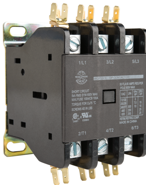
WDP 50 Series Contactor
