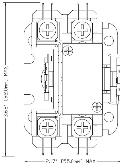
Front Detail
