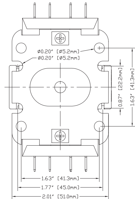
Base Detail
