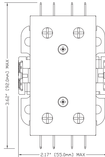
Front Detail
