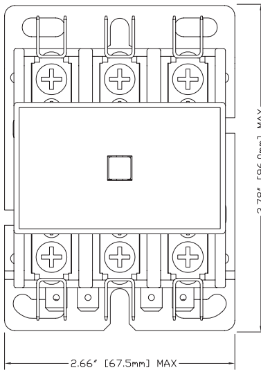
Front Detail
