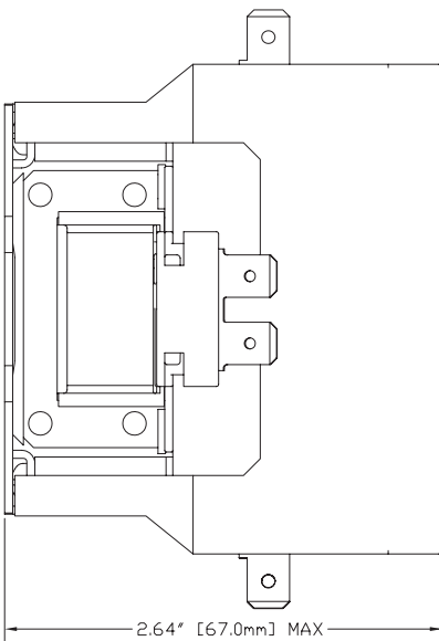
Side Detail
