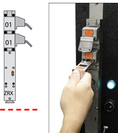
Pull trapped key from lock module. Machinery shuts down. Take trapped key to machinery gate (or door).
