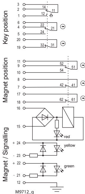
Fig. 1: Solenoid locking activated: Magnet locked, Key inserted
