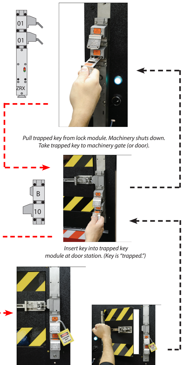
Keys trapped at main station (left). Door station with optional padlock module (right).
