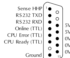
Port 0
