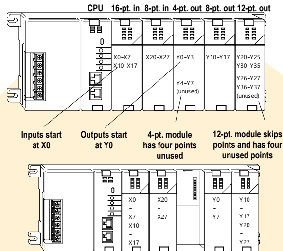
I/O base with a slot left empty. The examples below show the addressing changes if an input or an output module is added to the system.
