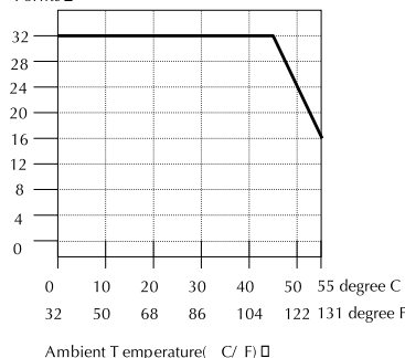
Derating Chart
