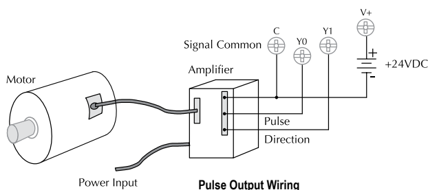
Equivalent Pulse Output Circuit Sinking Output
