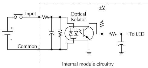
Equivalent Circuit, High-Speed Inputs
