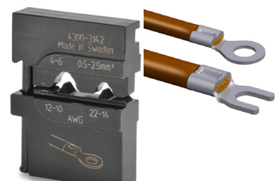
DN-CT-D3 (4300-3142) Non-Insulated Terminals & Connectors 22–10 AWG (0.5–6 mm 2 )
