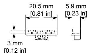
DN-MTA dimensions
