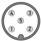
5-pin M12 Connector
