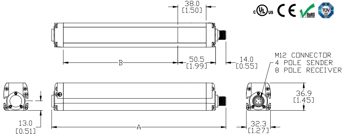
Receiver M12 8-pole male connector
