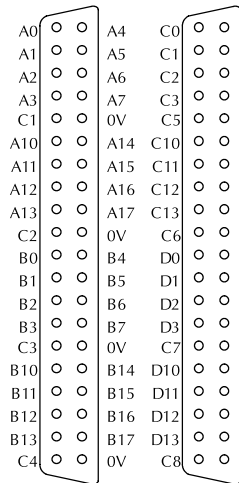
Connector Pins
