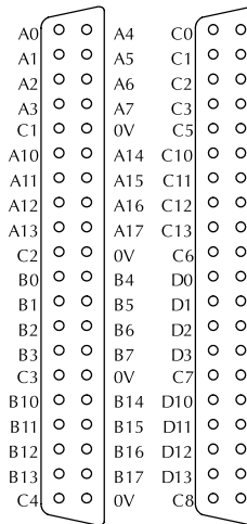
Connector Pins
