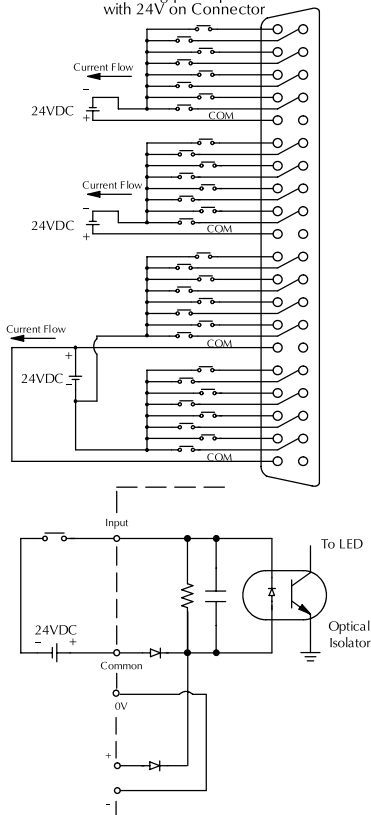
Wiring per 32pts. with 24V on Connector
