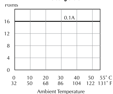
Derating chart
