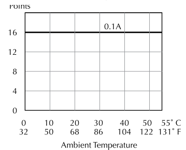
Derating chart
