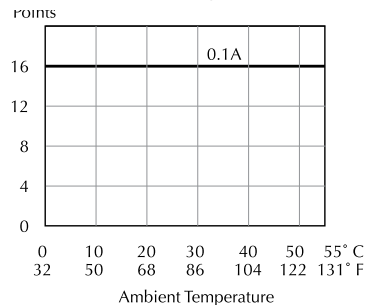
Derating chart
