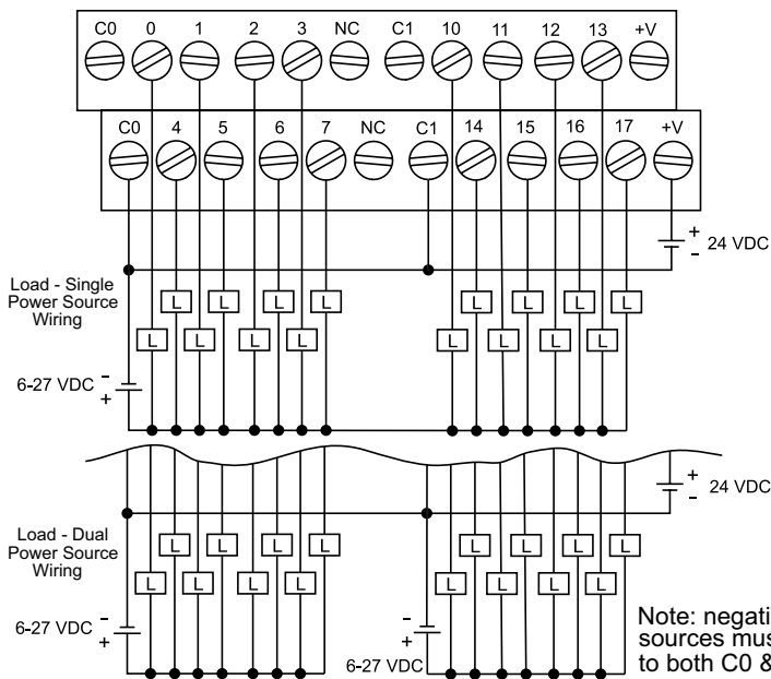
Typical Wiring Example
