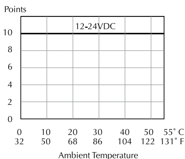
Derating chart
