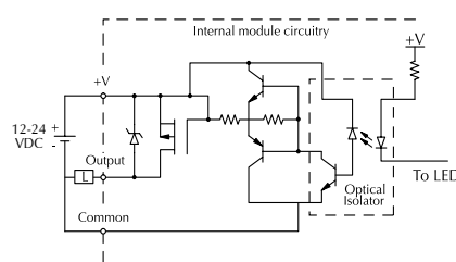
Equivalent output circuit Pulse output (Y0-Y1)
