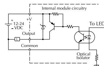
Equivalent output circuit Standard output (Y2-Y17)
