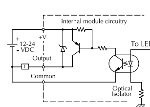
Equivalent output circuit Standard output (Y2-Y17)
