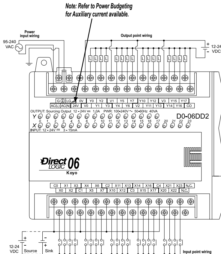
Equivalent input circuit, Standard inputs (X4-X23)
