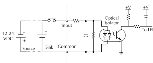
Equivalent input circuit, High-speed inputs (X0-X3)
