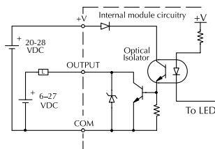
Equivalent output circuit Pulse output (Y0-Y1)
