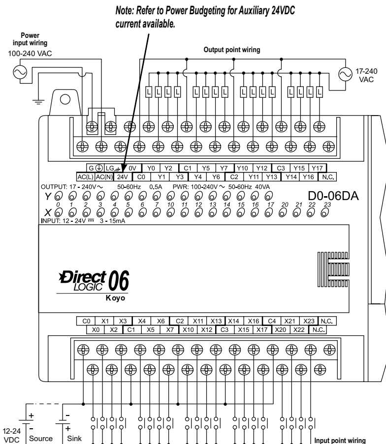
Equivalent input circuit, High-speed inputs (X0-X3)
