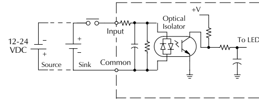
Equivalent input circuit, Standard inputs (X4-X23)
