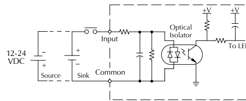
Equivalent input circuit, standard inputs (X3-X7)
