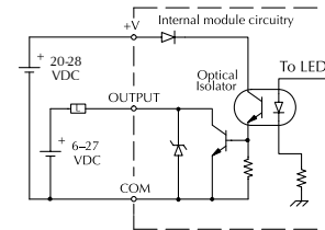
Equivalent output circuit standard outputs (Y2-Y5)
