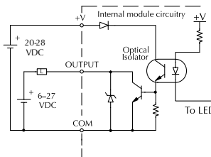
Equivalent output circuit pulse outputs (Y0-Y1)
