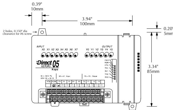
Mounting orientation
