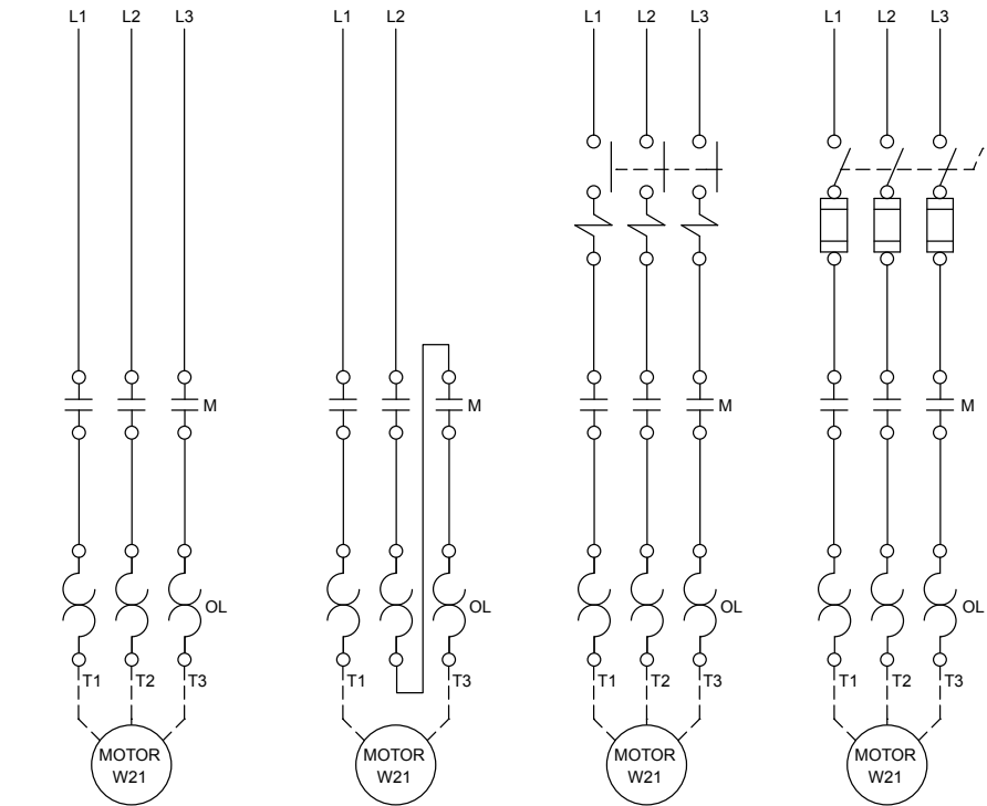
NON COMBINATION 3-PHASE NON COMBINATION 1-PHASE COMBINATION MCP COMBINATION FUS / NON FUS. DISC.
