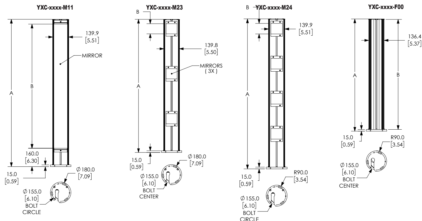
Safety Light Curtains Mirror Columns Dimensions
