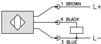
Diagram 1 PNP Output
