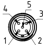
Plug M12, 5-pin
