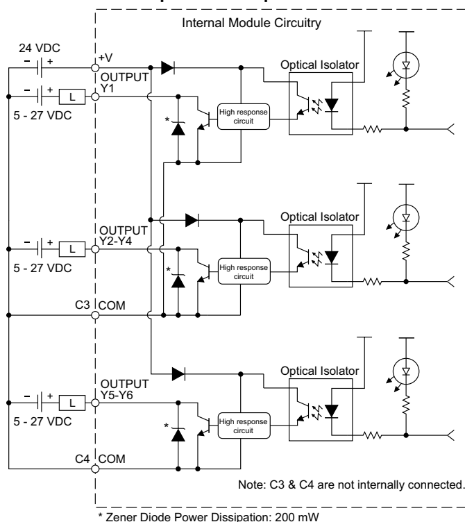
Equivalent Output Circuit
