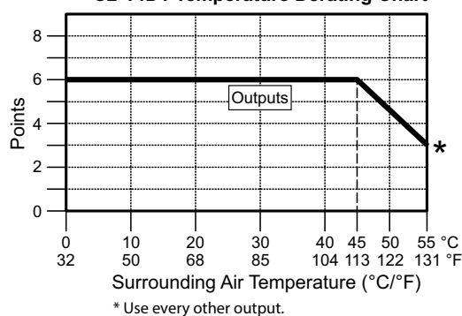
C2-14D1 Temperature Derating Chart
