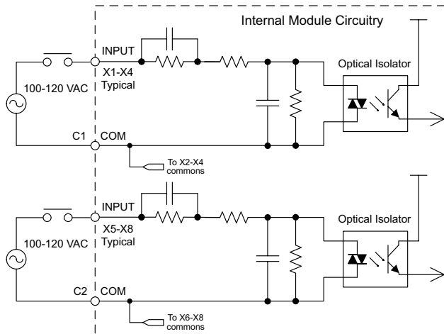
Equivalent Input Circuit
