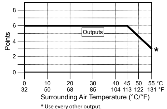
C2-14AR Temperature Derating Chart
