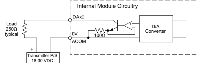
Analog Current Output Circuit
