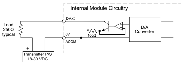
Analog Current Output Circuit
