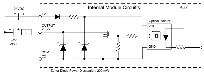
Equivalent Discrete Output Circuit
