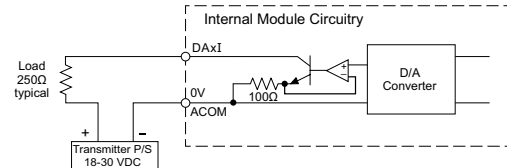
Analog Current Output Circuit
