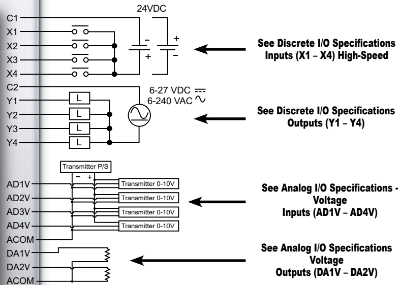
Wiring Diagram
