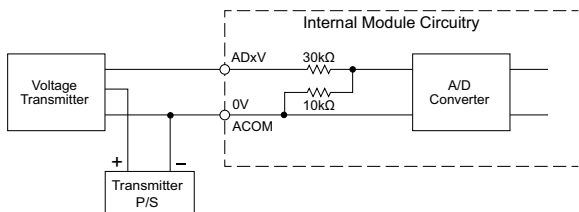
Analog Voltage Input Circuit
