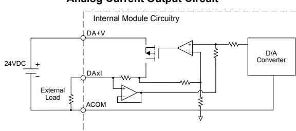
Analog Current Output Circuit
