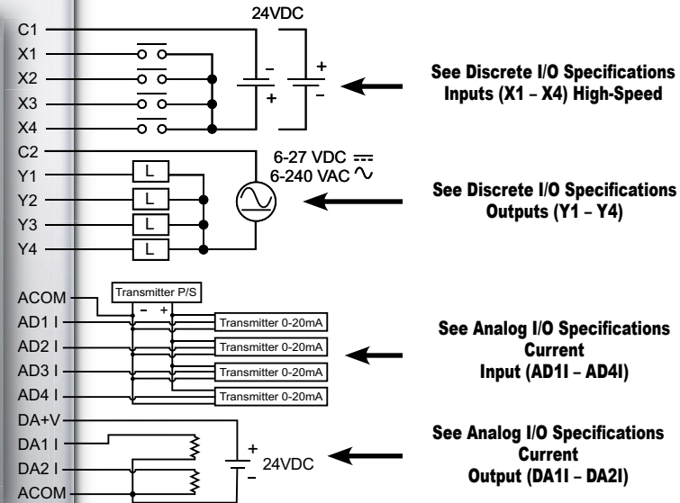
Wiring Diagram
